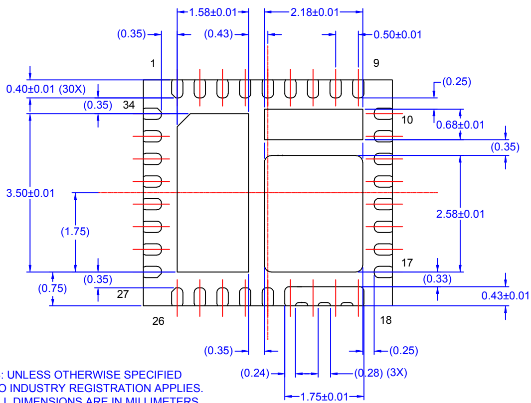
BOTTOM VIEW
